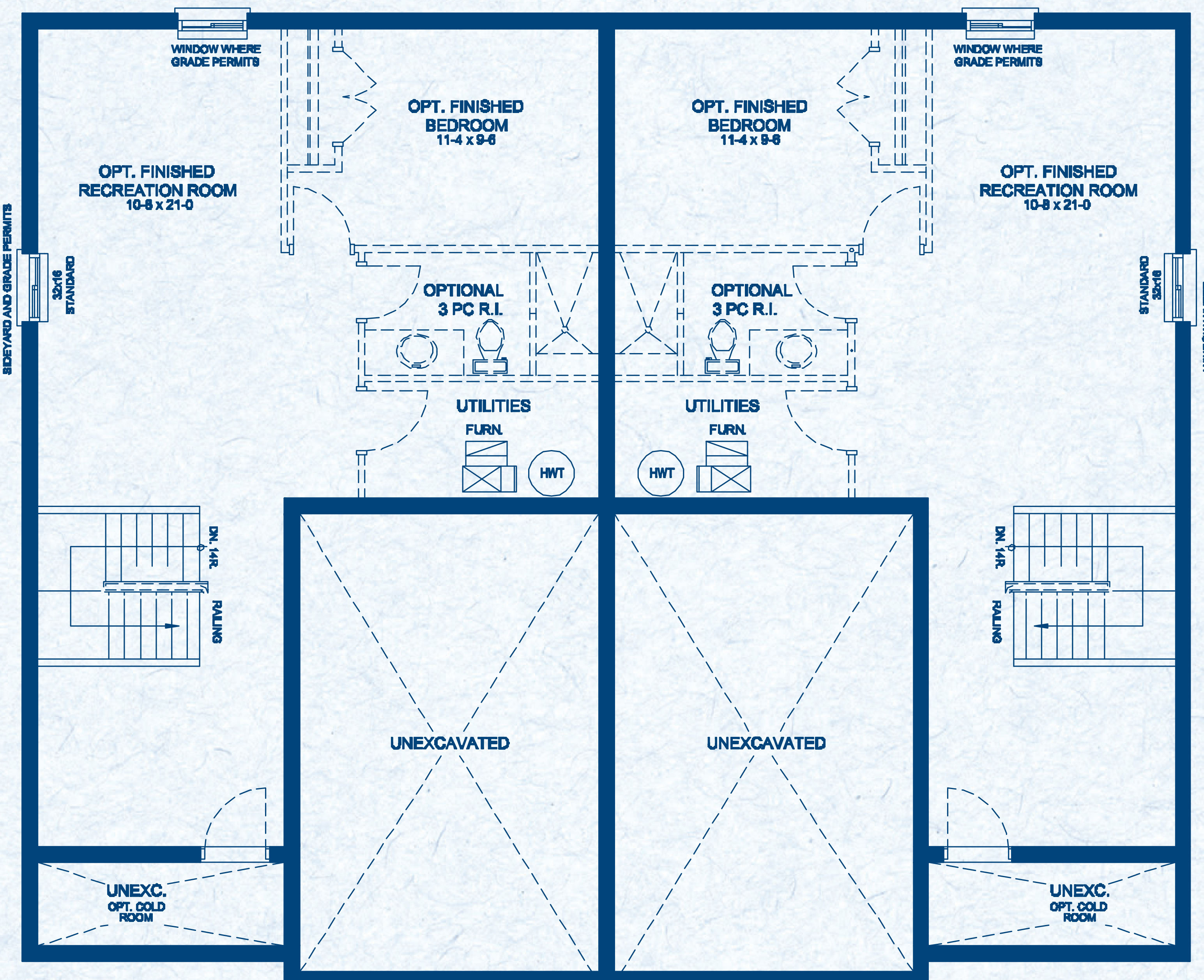
BASEMENT - B1 ELEVATION A
