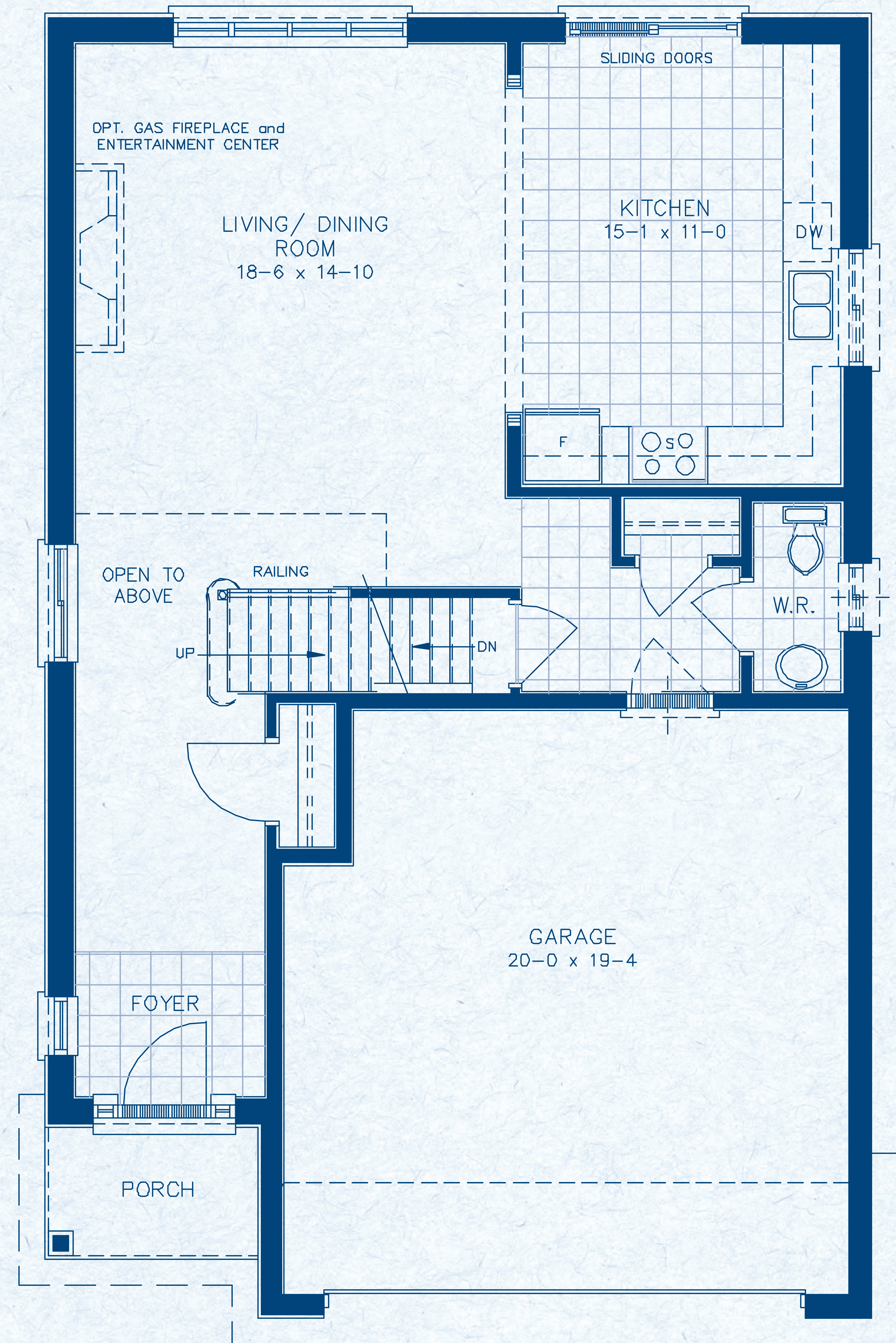
MAIN FLOOR - M1 ELEVATION A & B
