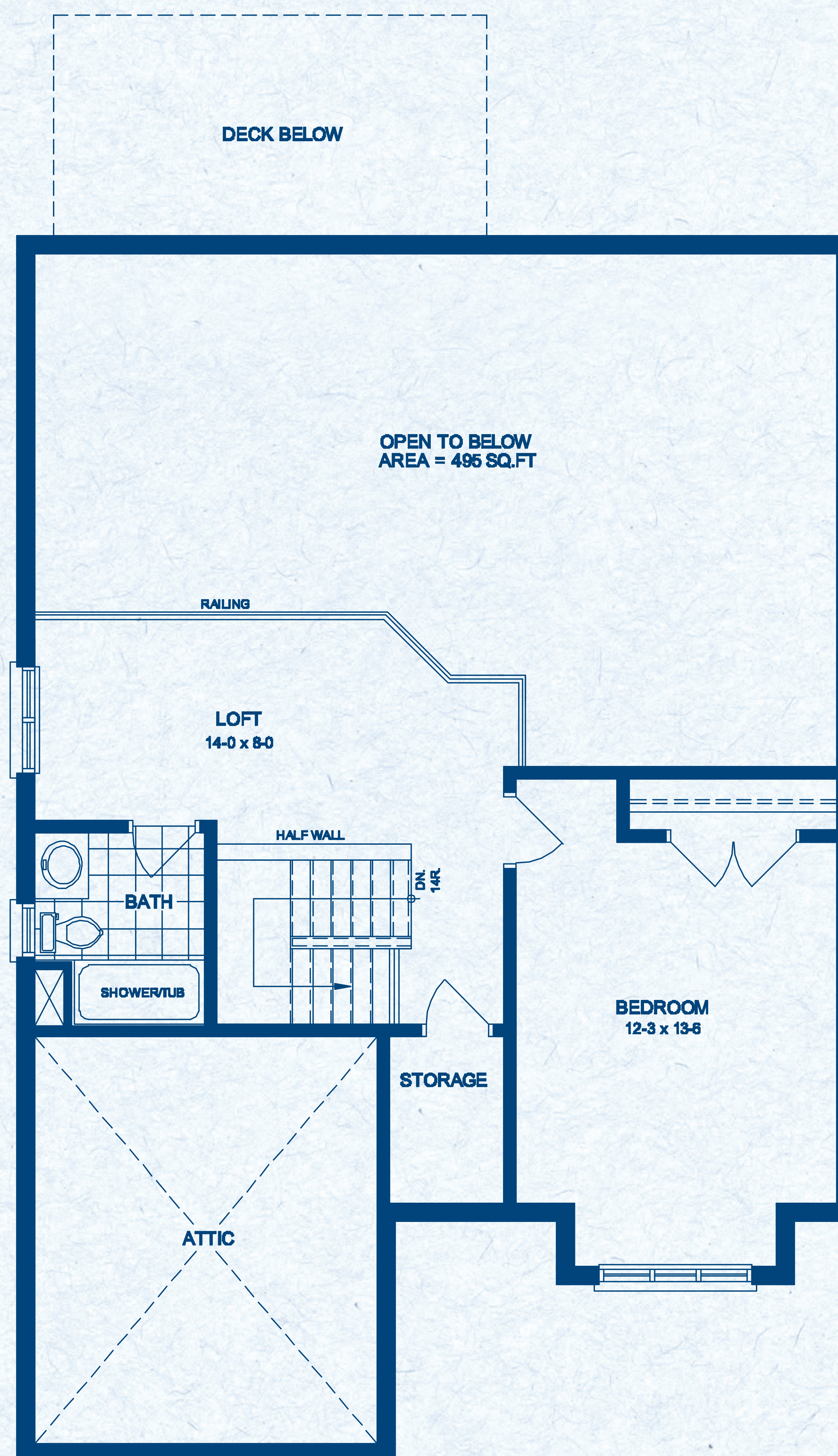
SECOND FLOOR - S1
