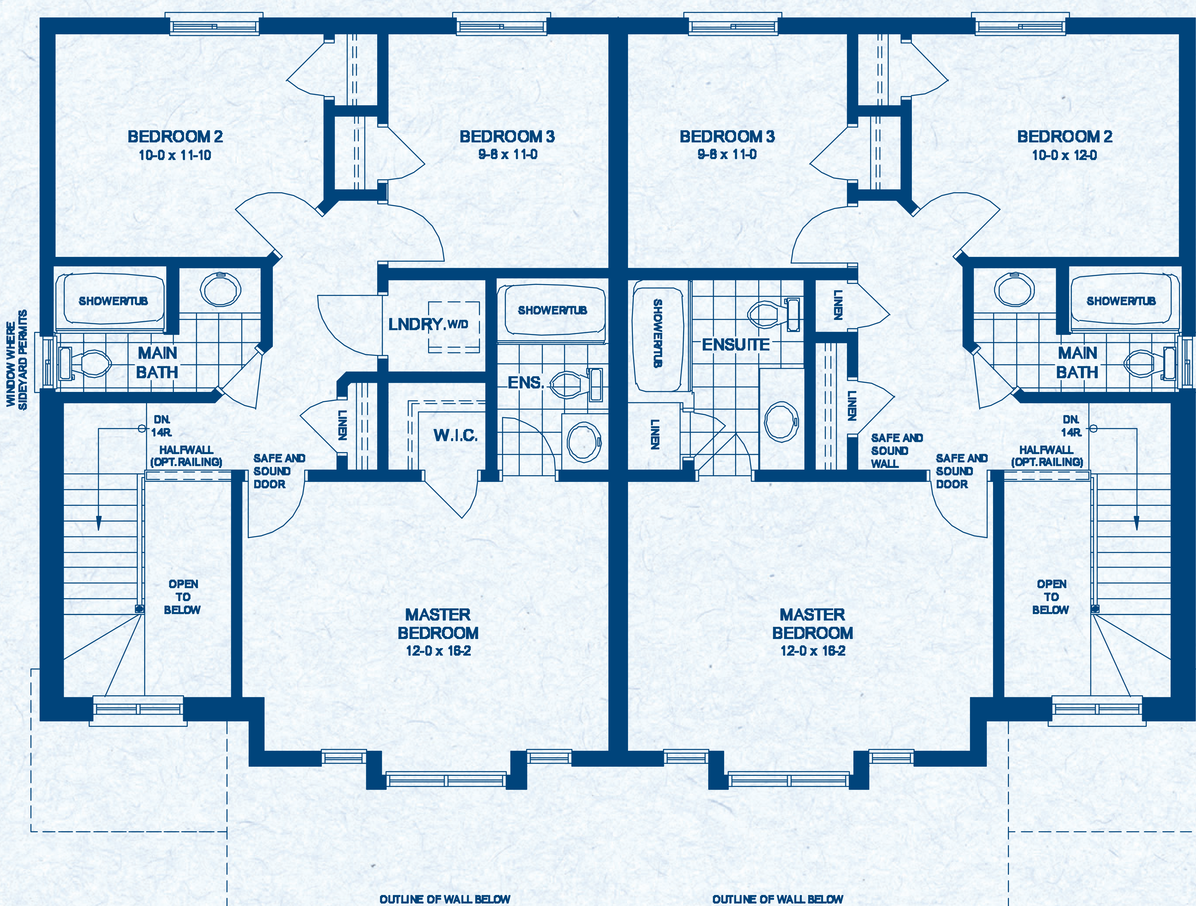
SECOND FLOOR - S1 ELEVATION A
