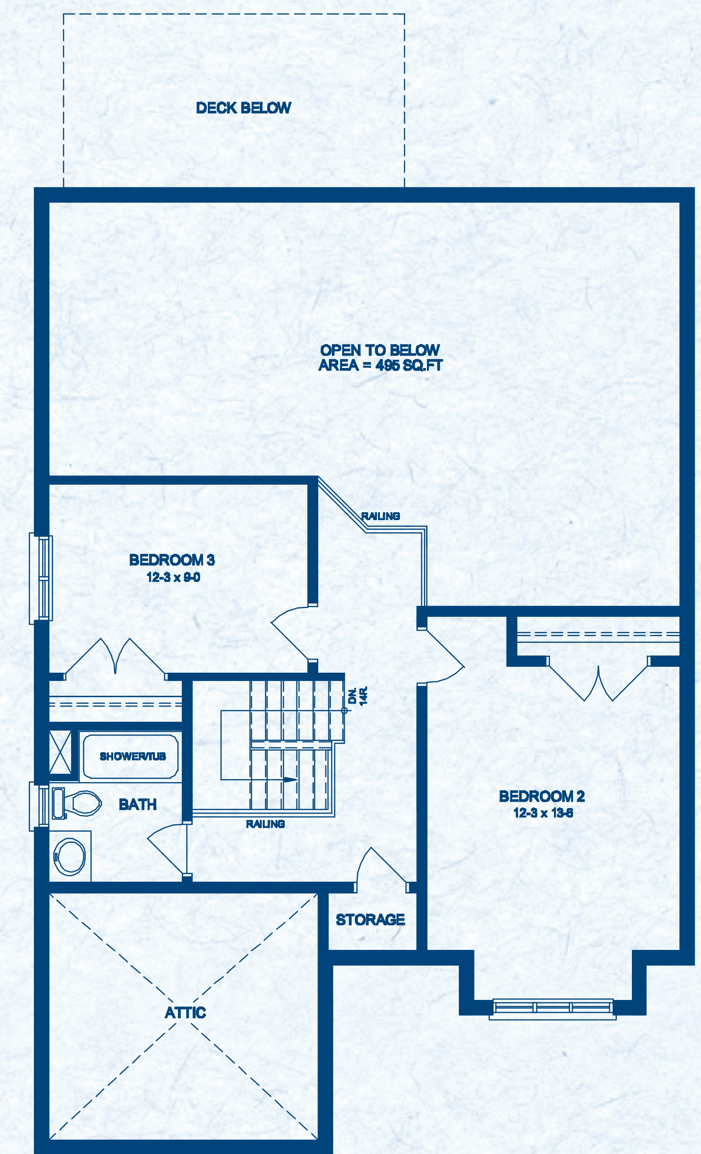
SECOND FLOOR - S2 OPTIONAL 3RD BEDROOM
