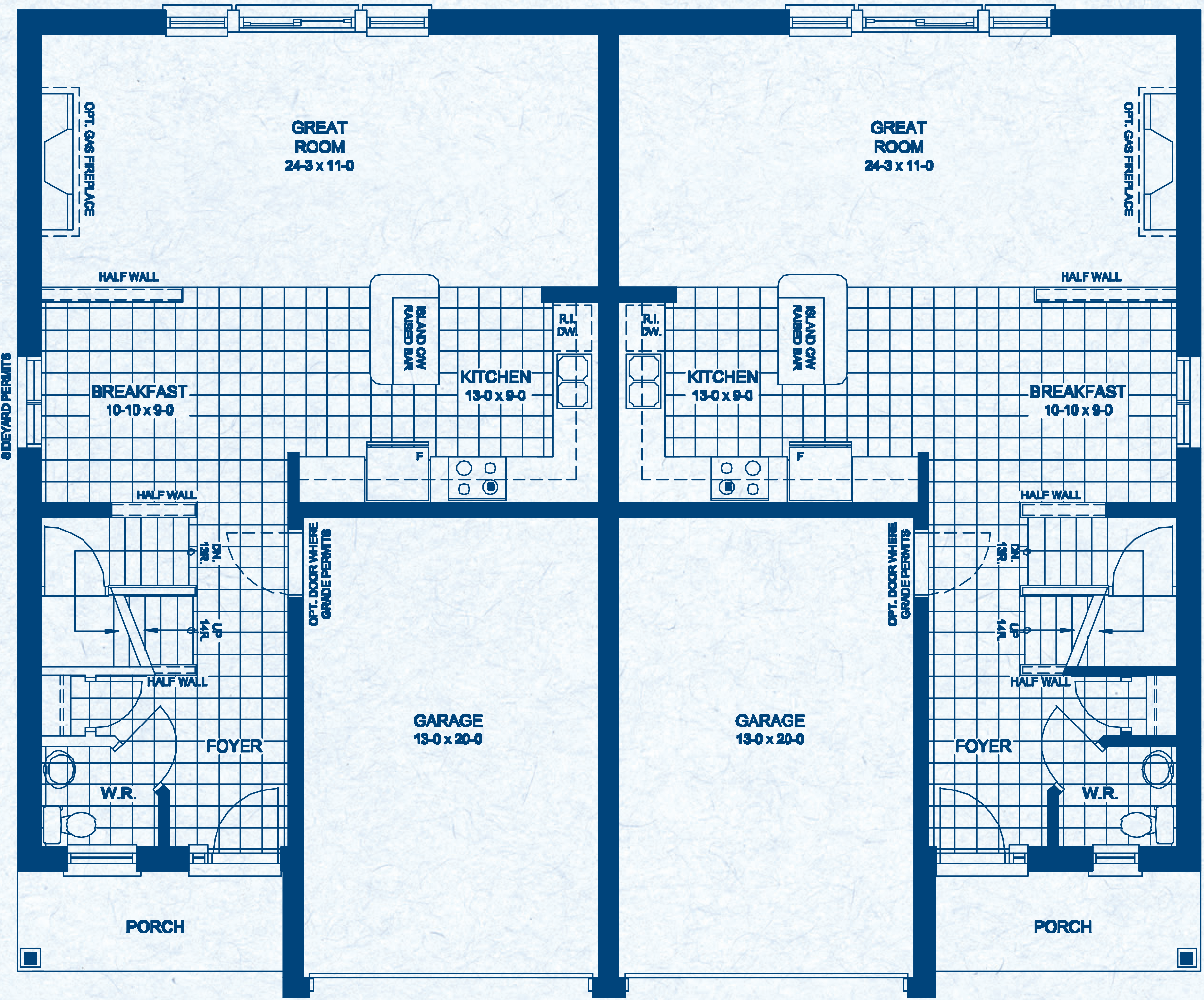
MAIN FLOOR - M1 ELEVATION A
