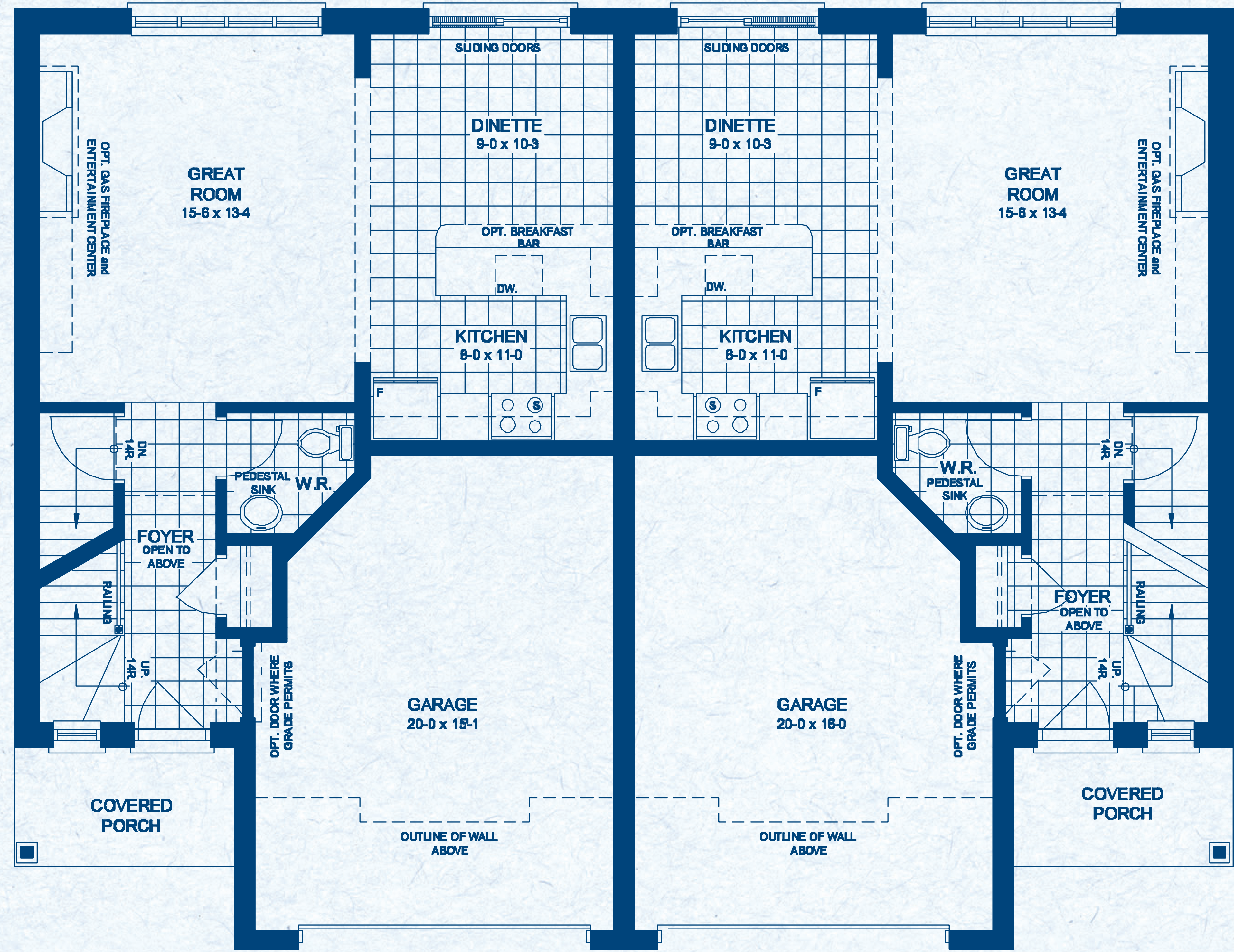
MAIN FLOOR - M1 ELEVATION A
