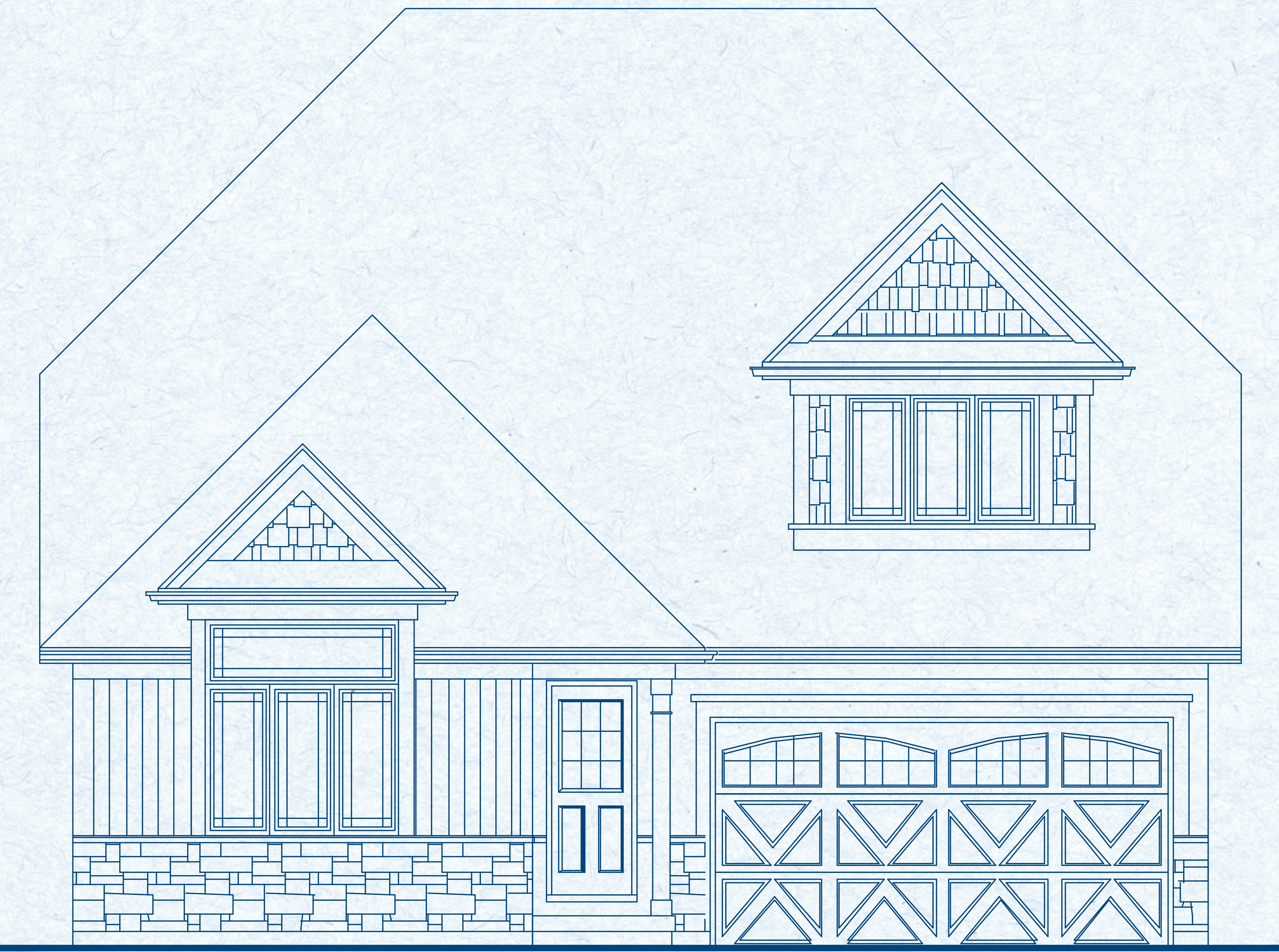
FRONT ELEVATION
