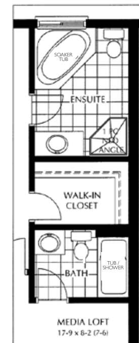
S2A – SECOND FLOOR
