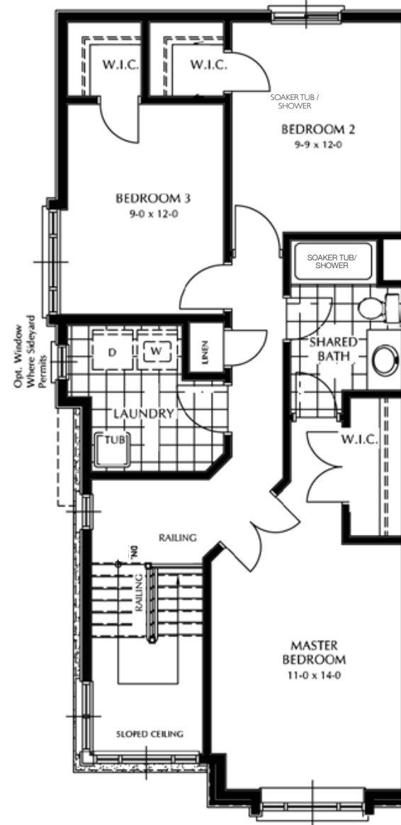
SECOND FLOOR – S1
