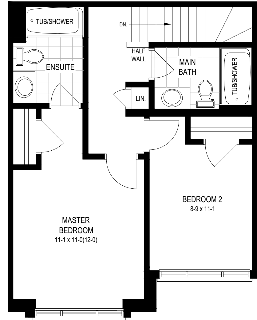
SECOND FLOOR w/ ENSUITE
