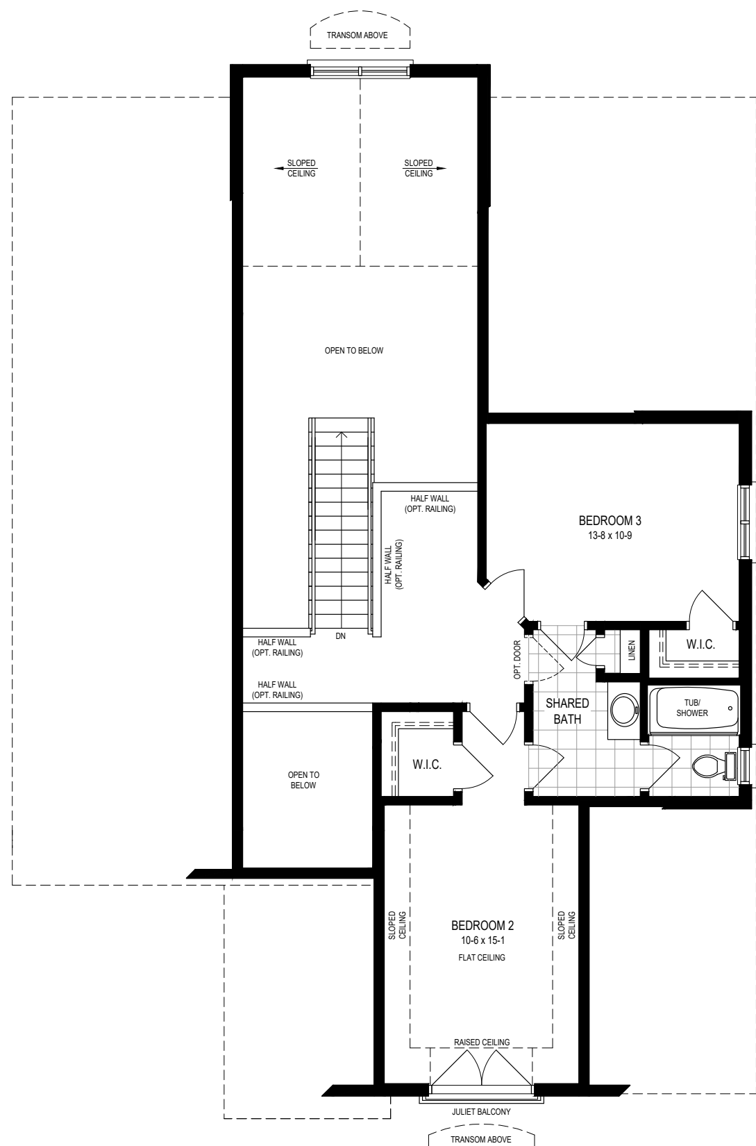
CHÂTEAU - S1, SECOND FLOOR
