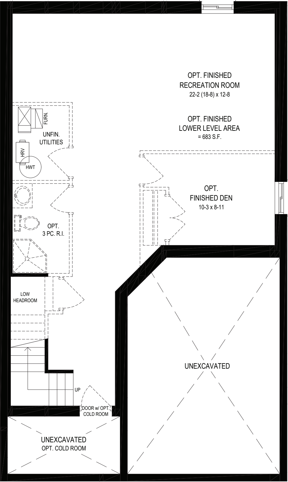
LOWER LEVEL
