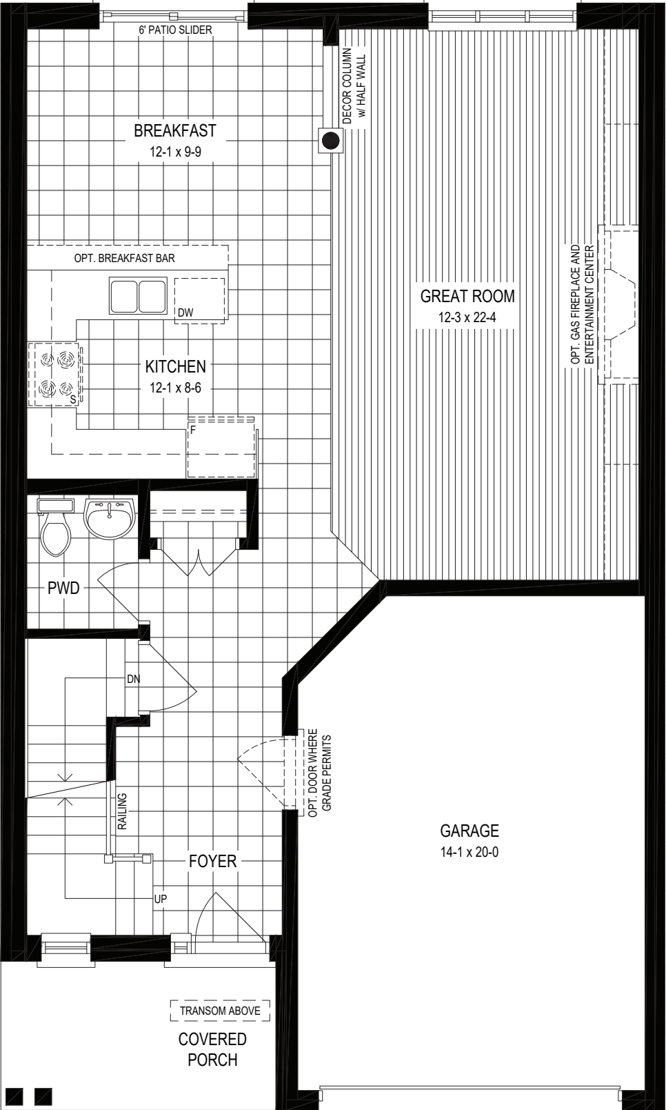
MAIN FLOOR
